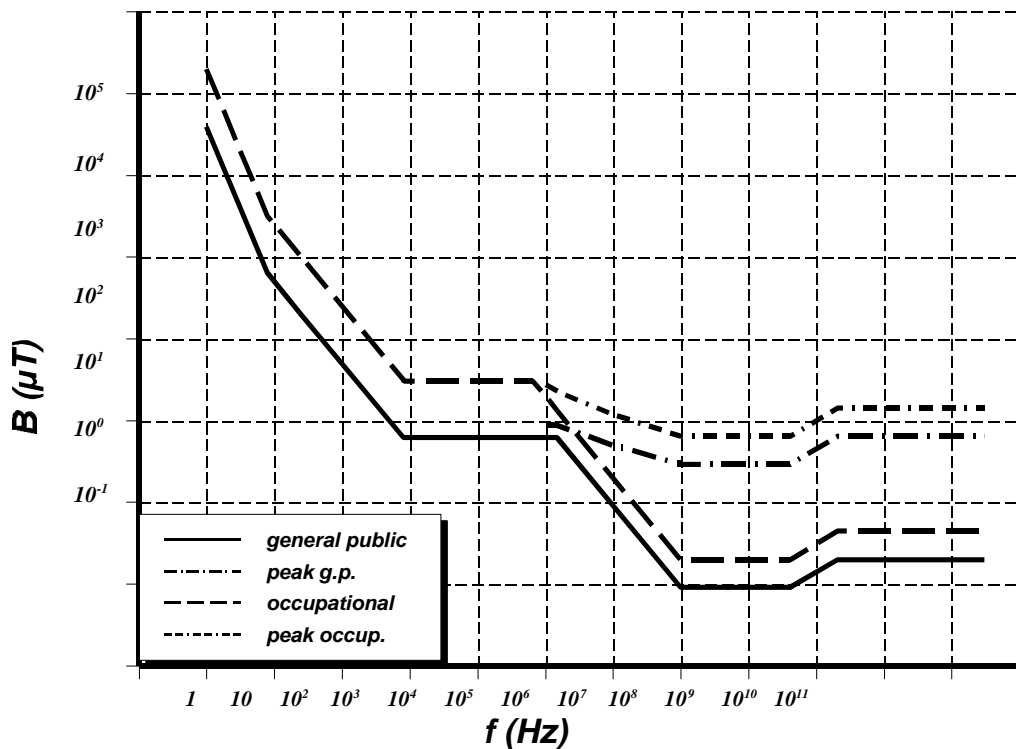
Figure 2 Reference levels for exposure to time varying magnetic fields (compare tables 6 and 7)
