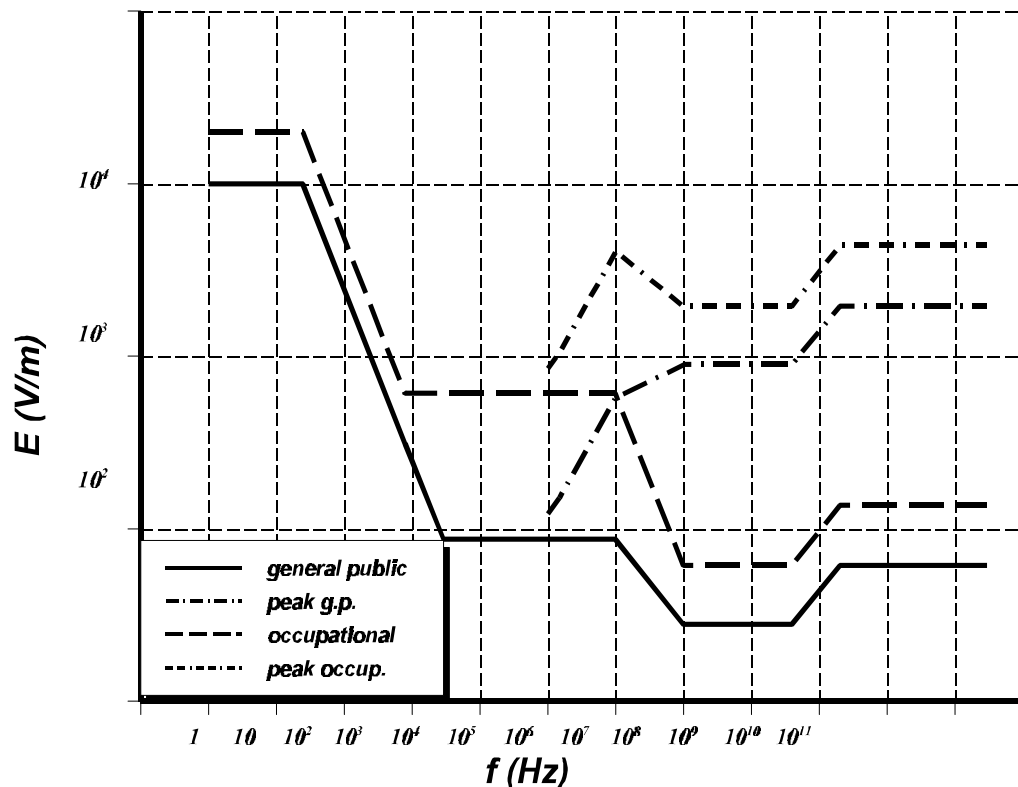
Figure 2 Reference levels for exposure to time varying electric fields (compare tables 6 and 7)
